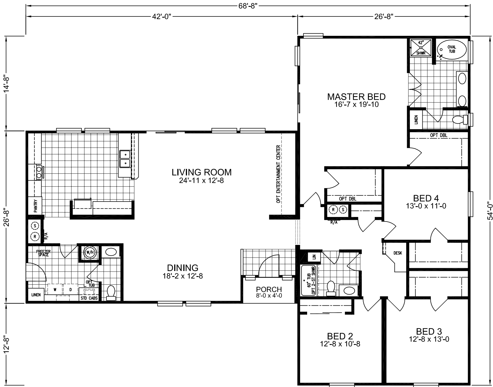
MODEL 688BT THE "MEADOW CREEK" APPROX. 2528 SQ. FT. 4 BEDROOM, 2 1/2 BATH
